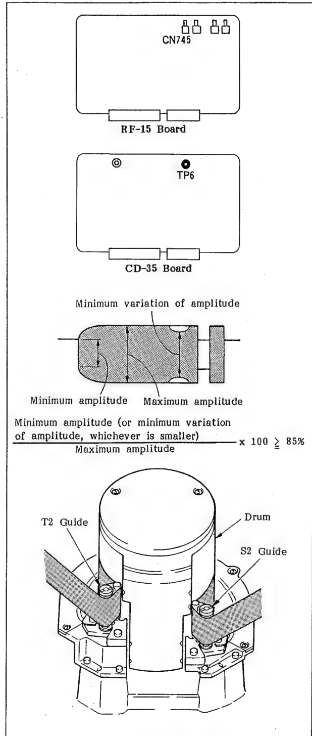
Fig. 9-11 Tracking Check
